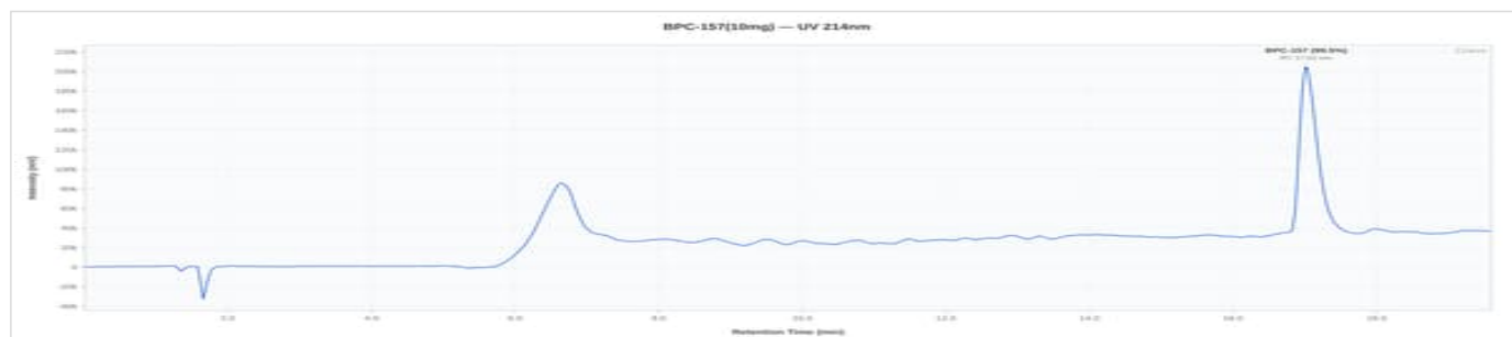
BPC-157 10mg - 2026723: UV Chromatogram
